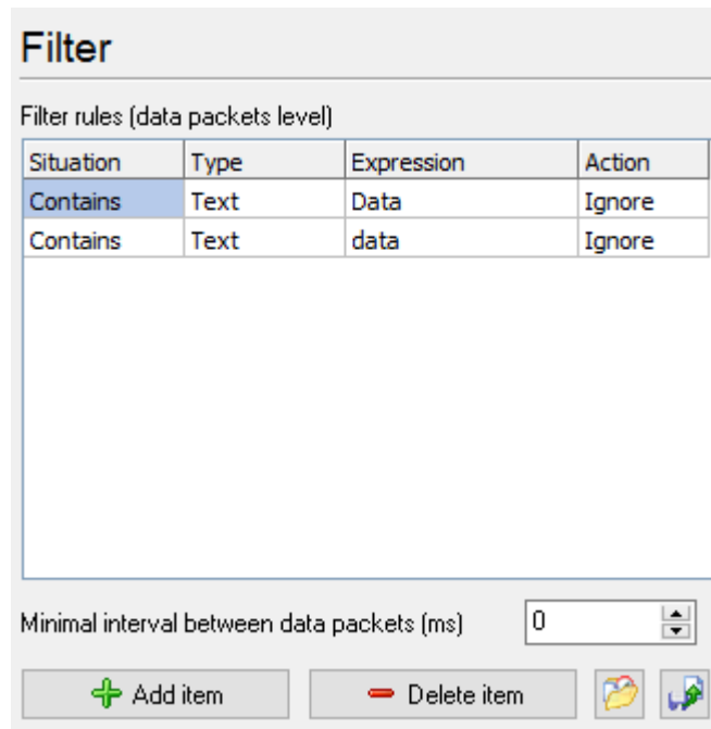
Fig. 2. Filtering rules
