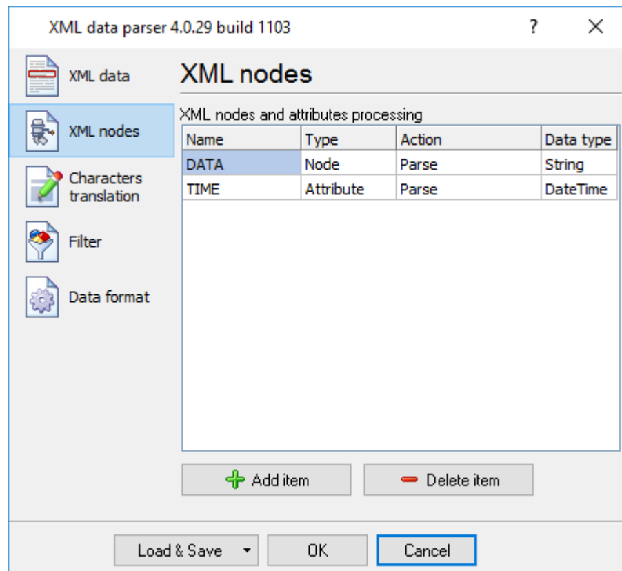
Fig.2. XML nodes.
