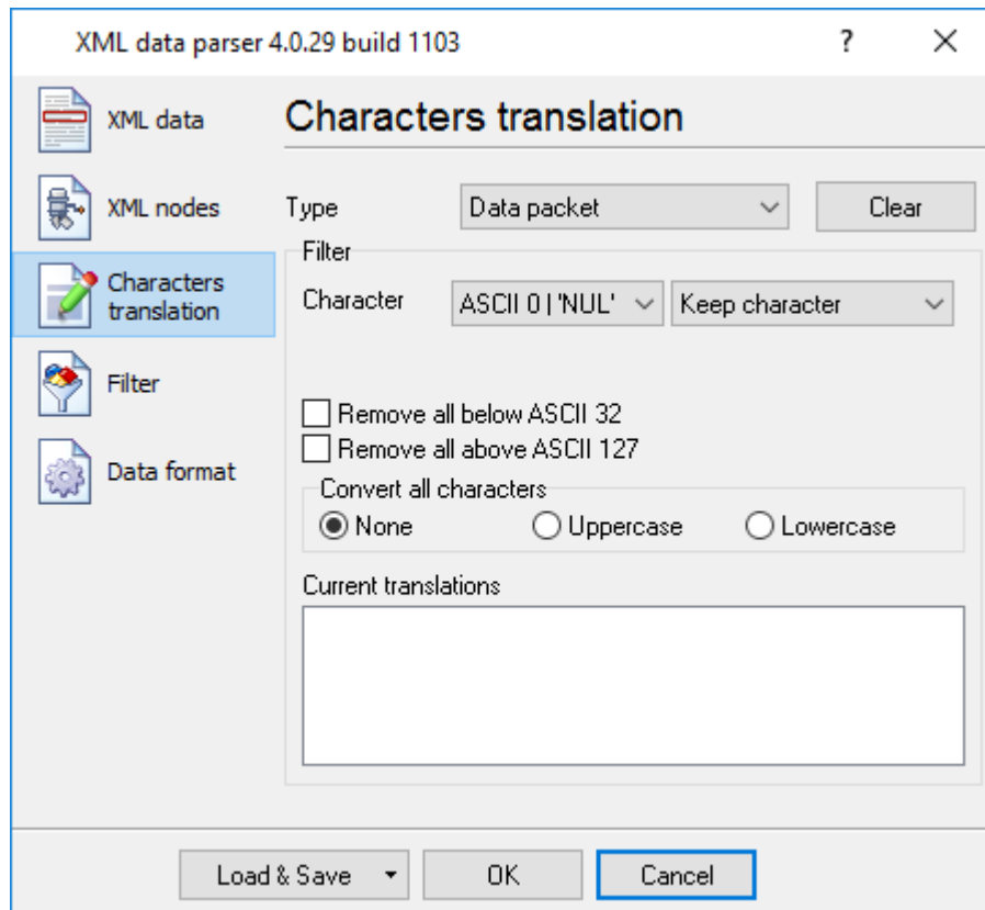
Fig.3 Character translation
