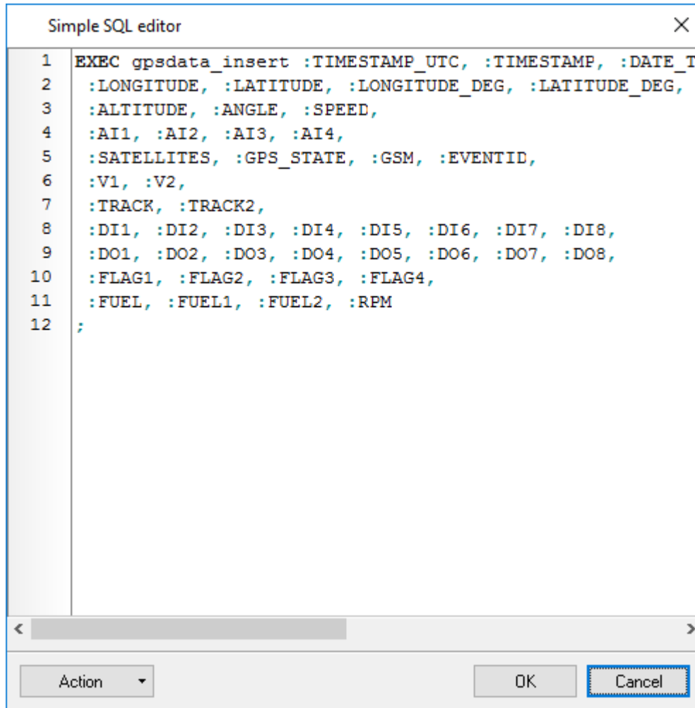
Fig. 6. SQL editor
