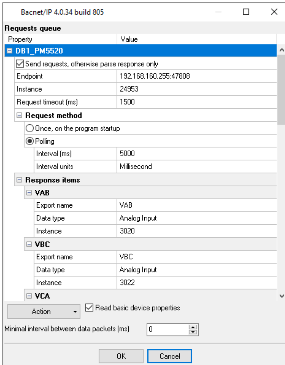
Figure 2: Request queue
